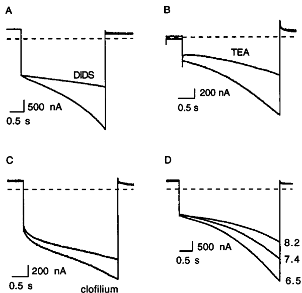
FIGURE 3 Pharmacology of the hyperpolarization-activated current. Effect of: (A) DIDS (1 mM), (B) TEA (100 \mu M), (C) clofilium (100 \mu M), (D) alteration of external pH. Oocytes injected with EAAT2 mRNA were recorded 4–7 days after injection in the absence of externally applied L-glutamate. Following a 3-s prepulse to 20 mV, currents were elicited by 3-s hyperpolarizing commands to -130 mV from a holding potential of -50 mV. To block residual calcium channels and screen surface charge, calcium was replaced by cobalt (1 mM) in the standard recording solution.
